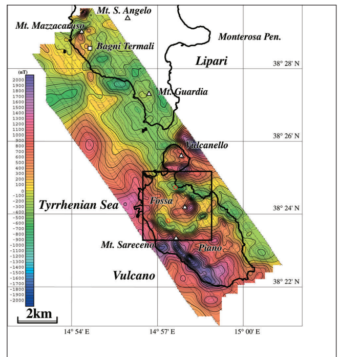
Fig. 4. Aeromagnetic anomaly (total magnetic intensity) map of Vulcano and Southern Lipari, compiled from the merged data from two aeromagnetic surveys which were flown at an altitude of 150 m above terrain with track lines spaced 250 m apart in October, 1999 and November, 2002, respectively. The observed data were reduced onto a smoothed surface 150 m above terrain on land and above sea level at sea. Contour interval is 50 nT. Open red circles indicate the locations of geothermal exploration wells.
