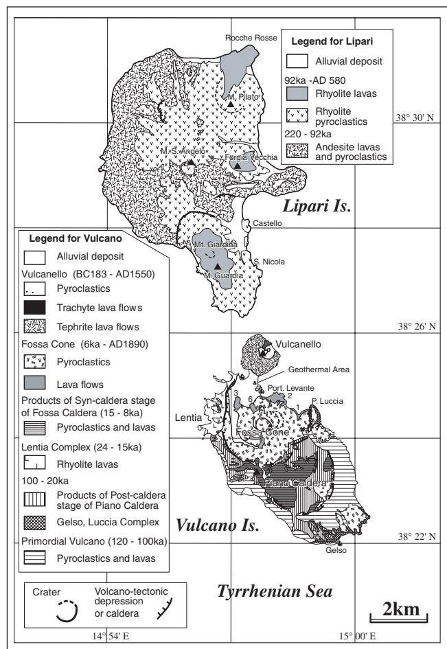
Fig. 3. Simplified geological map of Vulcano and Lipari Islands, Italy, modified from Pichler (1980) and Guest et al. (2003) for Lipari Island, and from Keller (1980) and De Astis et al. (1997) for Vulcano Island. Numbers from 1 to 6 on Vulcano correspond to lava flows — 1: Punta Roia (Tephrite), 2: Ponte Nere (Trachyte), 3: Campo Sportivo (Trachyte), 4: Palizzi (Trachyte), 5: Commenda (Rhyolitic Obsidian), 6: Pietre Cotte (Rhyolitic Obsidian).
