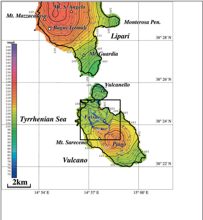
Fig. 7. Bouguer gravity map of Vulcano and Southern Lipari (Sugihara et al., 2002; Komazawa et al., 2003). Assumed density is 1.80 \times 10^3 \text{ kg/m}^3 . Contour interval is 1 mGal. Crosses indicate gravity stations.
