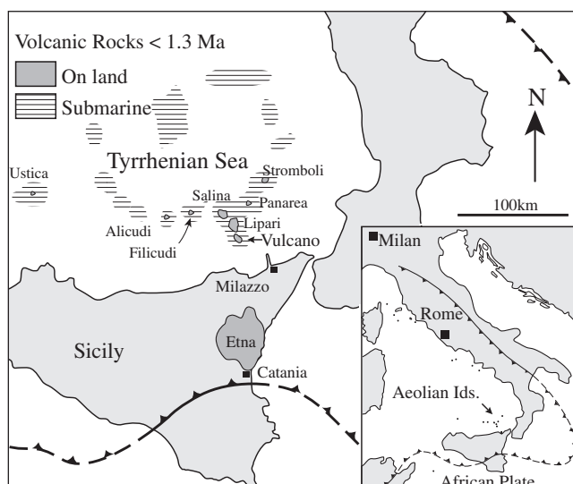
Fig. 1. The map of the study area shows the Aeolian Islands located between Sicily and the southern tip of the Italian Peninsula in the Tyrrhenian Sea. It also indicates the distribution of volcanic rocks of the age younger than 1.3 Ma (after Furukawa et al., 2000).
