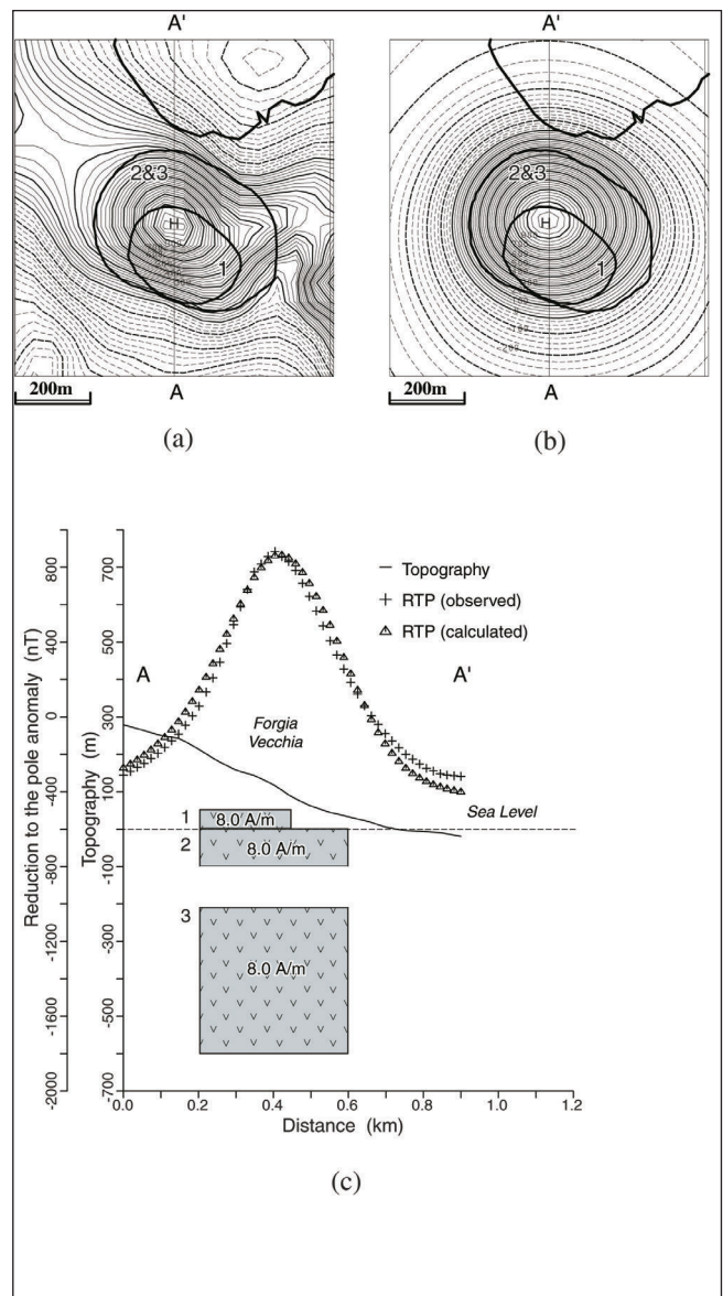
Fig. 9. Magnetic model of the Forgia Vecchia area. a) Reduction to the pole anomalies of the Forgia Vecchia area. Contour interval is 25 nT. The first-order regional trend was removed. Solid lines indicate the horizontal extent of the magnetic models (1-3). The thick solid line shows the coastline. The location of the area corresponds to A in Figure 8(a). See also Figure 8(a). b) Calculated reduction to the pole anomalies of the Forgia Vecchia area. (c) N-S cross section of the magnetic model of the Forgia Vecchia area.
